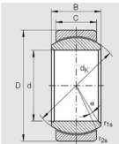
Spherical plain bearing 1 Outer ring 2 Sliding contact surface 3 Seal 4 Inner ring 5 Lubrication hole 6 Lubrication groove
